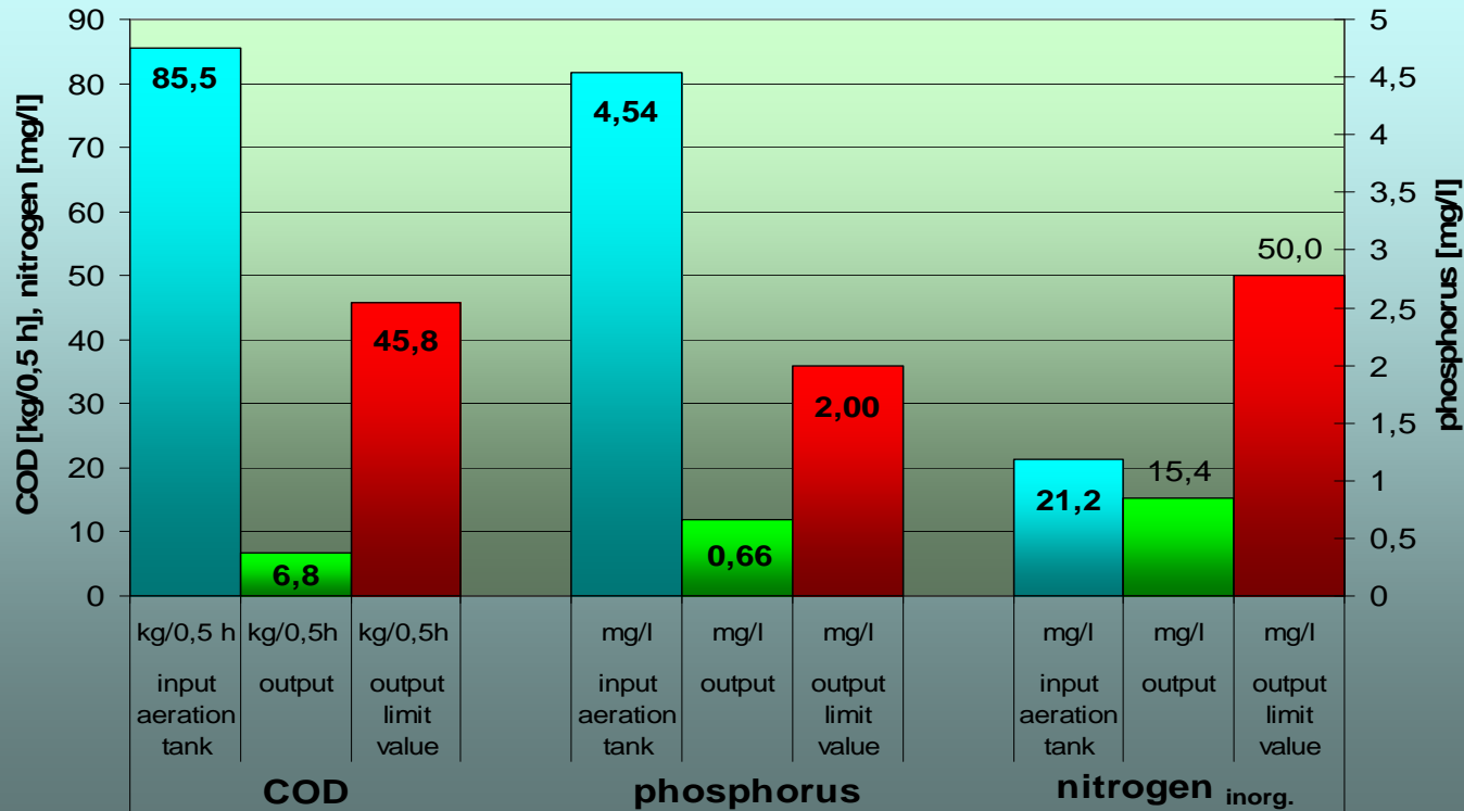
Waste water treatment plant Hürth average values for COD, phosphorus and nitrogen 2009
