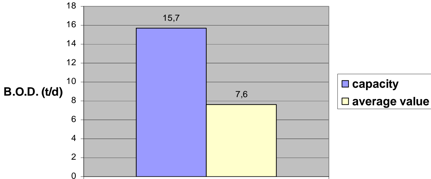
Wastewater treatment plants CPK B.O.D. - capacity and average values 2009
